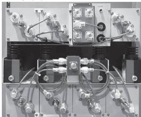
M104-150-4TPC in 19" rack
