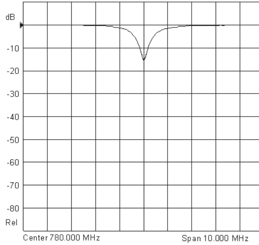
TYPICAL SELECTIVITY CHARACTERISTICS
