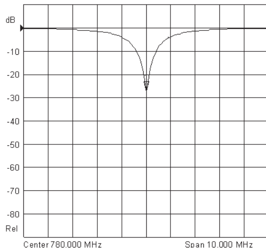
TYPICAL SELECTIVITY CHARACTERISTICS
