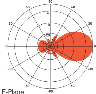
E-Plane Gain: 10.2 dBd
