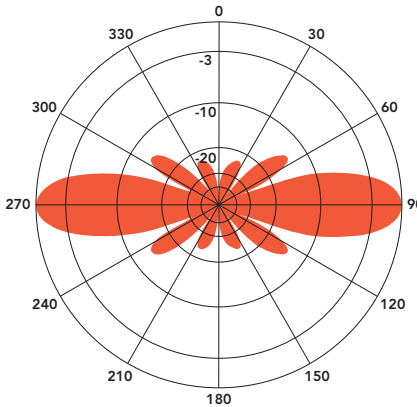
ANT940F6 - 930 MHz Vertical Plane Gain = 6.1 dBd
