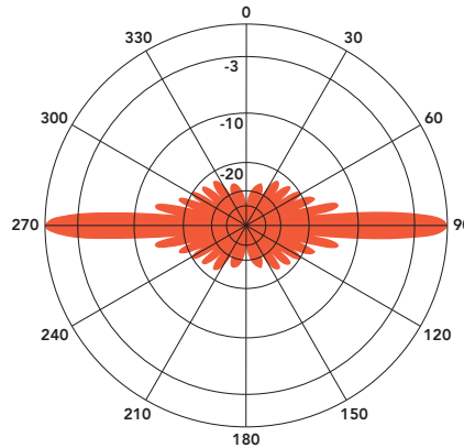
ANT940F10 - 830 MHz Vertical Plane Gain = 10.12 dBd
