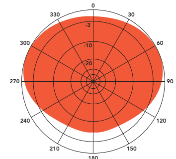
H-Plane, Gain = 1.9 dBd Spaced 3/8 wl. from mast
