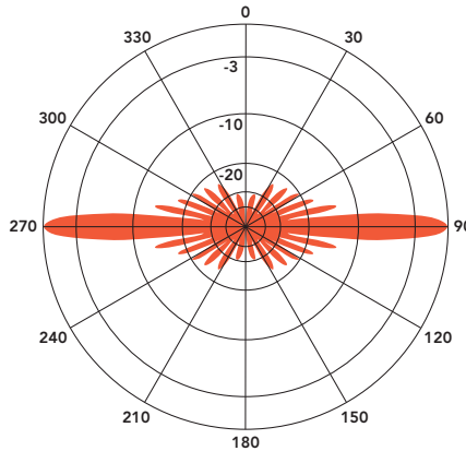
ANT450F10 - 450 MHz Vertical Plane Gain = 10.06 dBd
