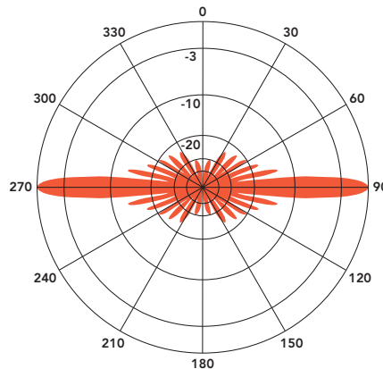
ANT500F10 - 495 MHz Vertical Plane Gain = 10.06 dBd
