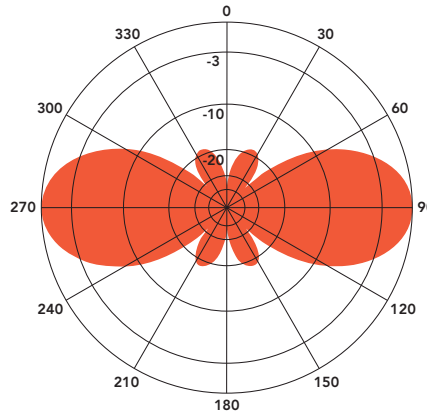
ANT770F2 - 750 MHz Vertical Plane Gain = 2.5 dBd
