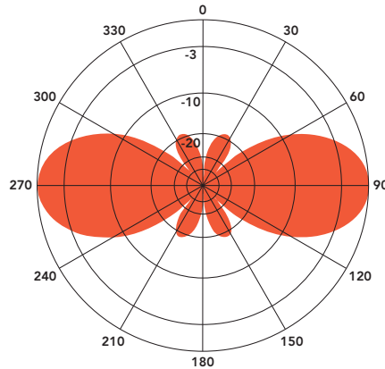
ANT850F2 - 851 MHz Vertical Plane Gain = 2.58 dBd
