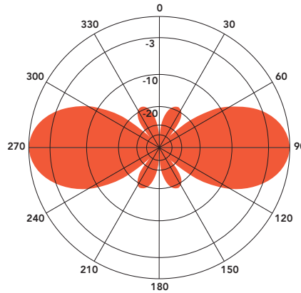
ANT900F2 - 928 MHz Vertical Plane Gain = 2.5 dBd
