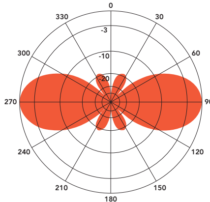
ANT734-960F2 - 838 MHz Vertical Plane Gain = 2.5 dBd
