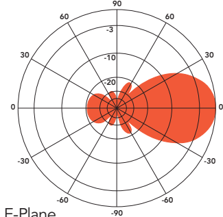
ANT850Y10-WR at 877 MHz
