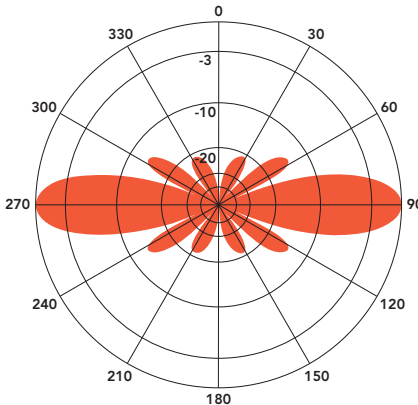
ANT355F6 - 355 MHz Vertical Plane Gain = 6.27 dBd
