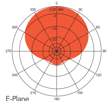
E-Plane Gain: 5.2 dBd
