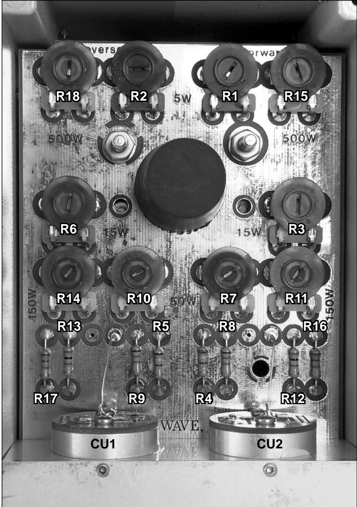
Figure 6-1: Adjustment Potentiometers and Parts Location
