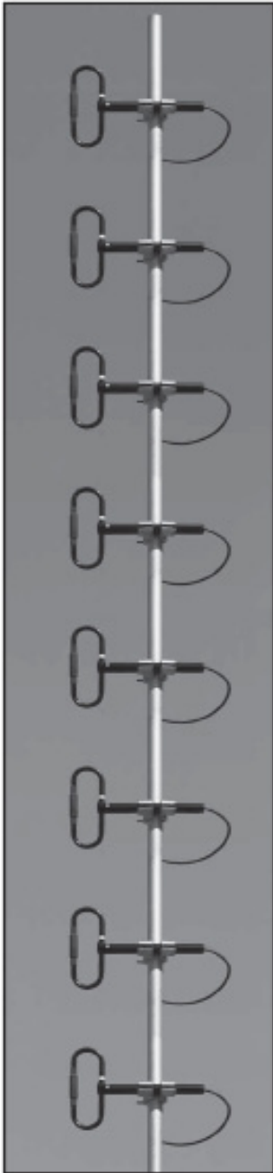
ANT500D7 - 12 (Harness not shown) Support mast is customer-supplied
