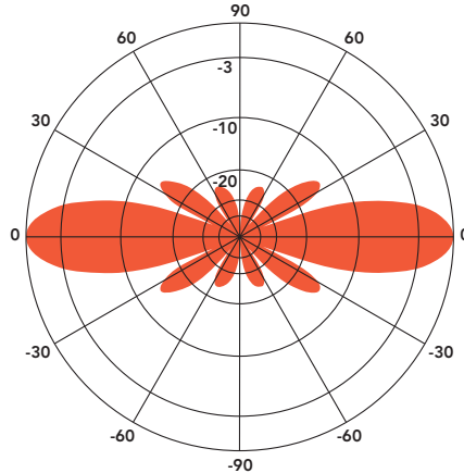
ANT385F6 - 385 MHz Vertical Plane Gain = 6.12 dBd
