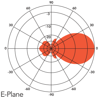
ANT490Y10-WR at 490 MHz
