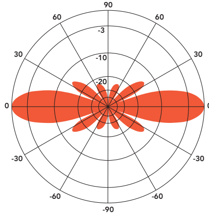
ANT395F6 - 395 MHz Vertical Plane Gain = 6.12 dBd
