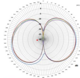
Vertical Beam Pattern
