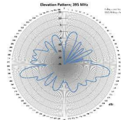
Vertical Beam Pattern 395 MHz
