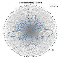
Vertical Beam Pattern 425 MHz
