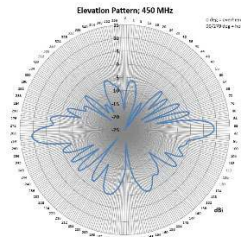
Vertical Beam Pattern 450 MHz
