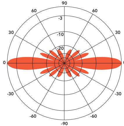
ANT415F6 - 421 MHz Vertical Plane Gain = 6.7 dBd
