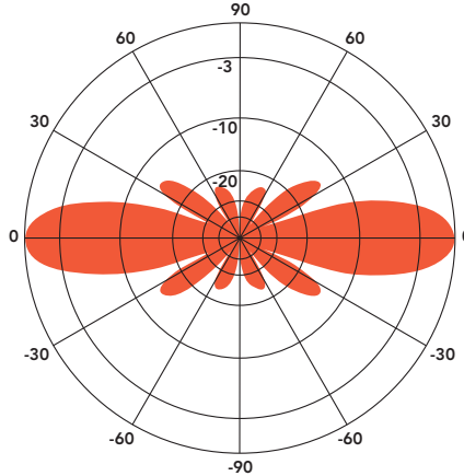
ANT830F6 - 800 MHz Vertical Plane Gain = 6.10 dBd
