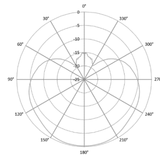
Average Vertical Pattern
