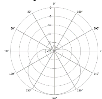
Average Horizontal Pattern
