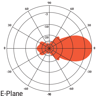
E-Plane Gain: 12.0 dBd
