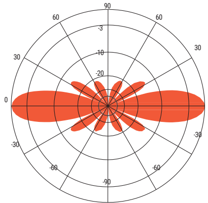
ANT355F6 - 355 MHz Vertical Plane Gain = 6.27 dBd
