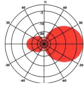
E-Plane Gain: 7.15 dBd
