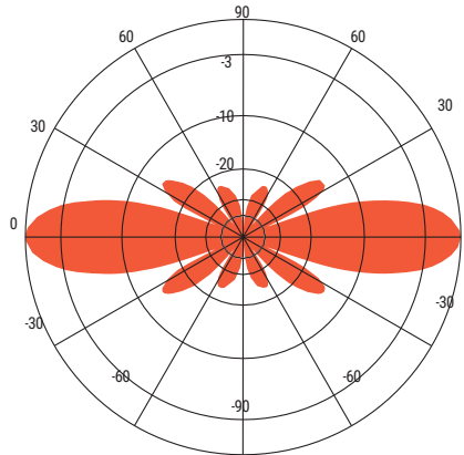
ANT385F6 - 385 MHz Vertical Plane Gain = 6.12 dBd
