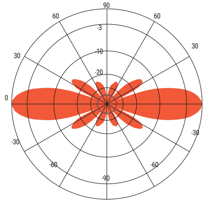
ANT395F6 - 395 MHz Vertical Plane Gain = 6.12 dBd
