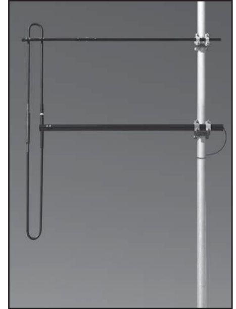
ANT40D at 40 MHz
