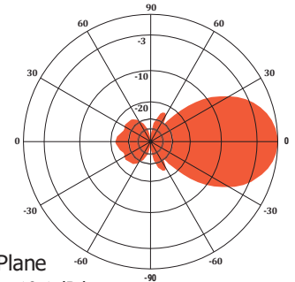
ANT410Y10-WR at 410MHz
