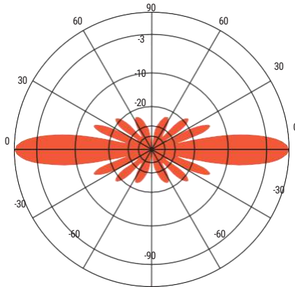
ANT415F6-421 MHz Vertical Plane Gain = 6.7 dBd
