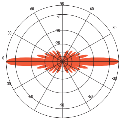
ANT415F8 - 420 MHz Vertical Plane Gain = 8.68 dBd
