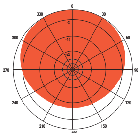
H-Plane gain 9.02 dBd 1/4 wl. spacing from tower
