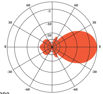
E-Plane Gain: 10.1 dBd
