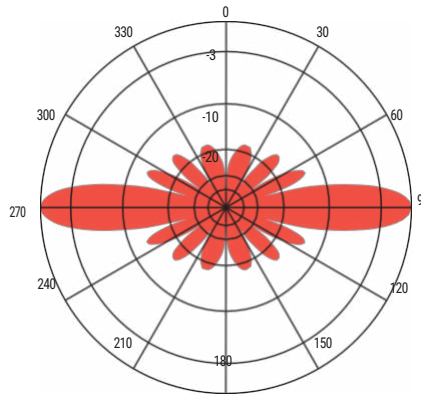
ANT440F6-450 MHz Vertical Plane Gain = 6.22 dBd
