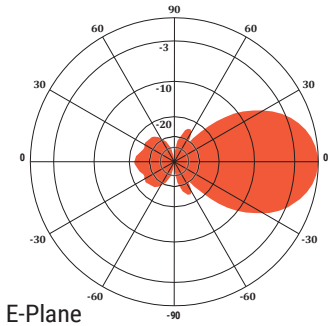
ANT440Y10-WR at 440 MHz
