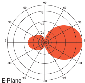
ANT450Y7-WR at 460 MHz
