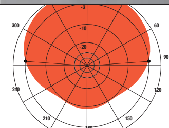
H-Plane gain 2.6 dBd 1/4 wl. spacing from tower
