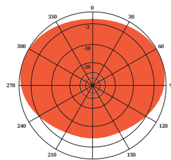
H-Plane gain 12.7 dBd 3/8 wl. spacing from tower
