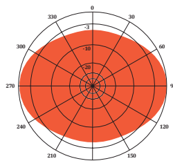
H-Plane gain 11.8 dBd 1/2 wl. spacing from tower
