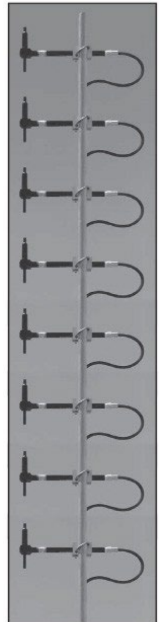
ANT750D7 - 12 (Harness not shown) Support mast is customer-supplied
