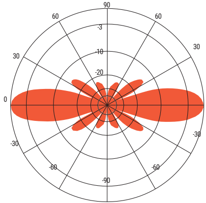
ANT770F6 - 776 MHz Vertical Plane Gain = 6.15 dBd
