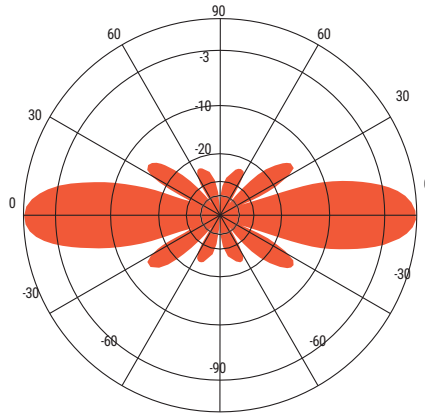
ANT825F6 - 800 MHz Vertical Plane Gain = 6.09 dBd
