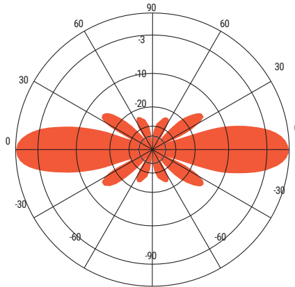
ANT830F6 - 800 MHz Vertical Plane Gain = 6.10 dBd
