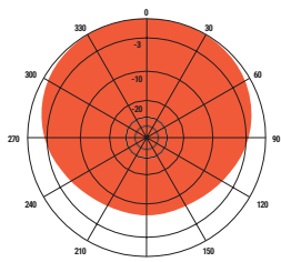
H-Plane gain 12.2 dBd 1/4 wl. spacing from tower
