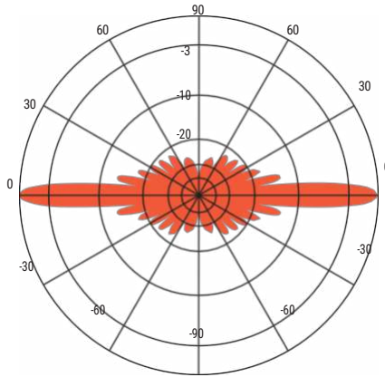
ANT940F10 - 930 MHz Vertical Plane Gain = 10.12 dBd
