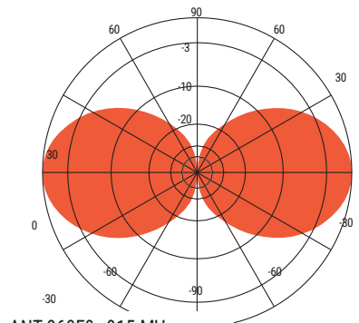
ANT 960F0 - 915 MHz Vertical Plane Gain=0dBd
