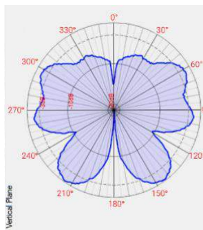
Vertical Beam Pattern (450 MHz)
