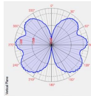
Vertical Beam Pattern (410 MHz)
