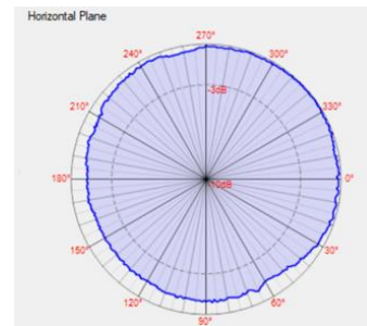
Horizontal Beam Pattern
