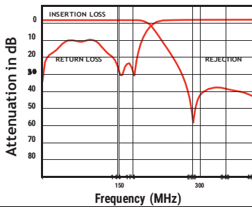
TYPICAL RESPONSE CURVE - TLF-150
